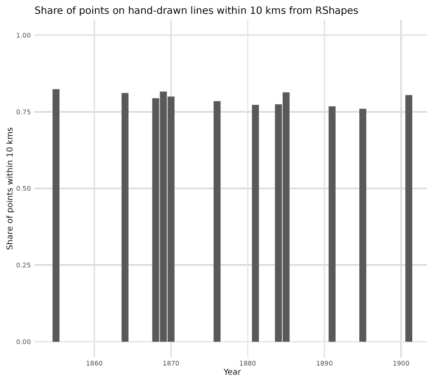
Figure A3: Similarity statistics of RShapes and Austro-Hungarian railway data.
