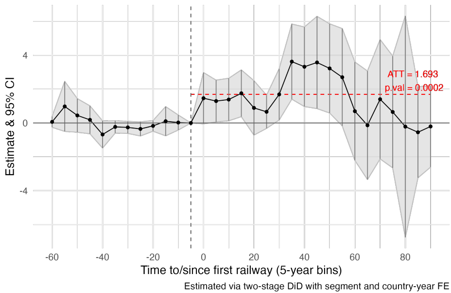
Figure 3: Event study plots (ATT estimates based on Columns 3 and 4 in Table 1)
